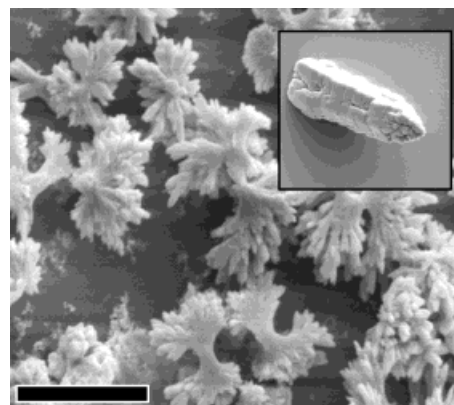
Figure 4. Scanning electron micrograph of \text{SrCO}_3 crystals precipitated from solutions containing the colloid seeds ( 30 \text{ mg L}^{-1} at 4^\circ\text{C} ). The scale bar corresponds to 10 \mu\text{m} . The inset shows a needle (ca. 15 \mu\text{m} long) of \text{SrCO}_3 in the strontianite modification obtained from precipitation in the absence of colloids. The needle grows along a pseudohexagonal [001] trilling axis.
