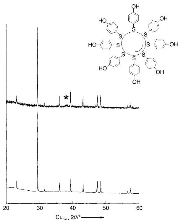
Figure 1. Measured and Rietveld-fitted X-ray diffraction profiles (transmission, \theta-2\theta ) of \text{CaCO}_3 crystallized from solutions containing thiol-coated gold colloid seeds. The fit indicates pure calcite; the small hump marked by an asterisk is due to the (111) reflection of gold. The concentration of seeds used was 100 \text{ mg L}^{-1} in solution, and the crystallization was carried out at 22^\circ\text{C} .
