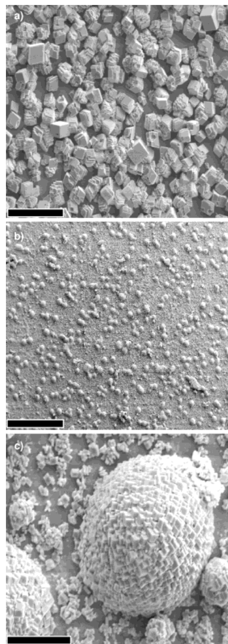
Figure 2. a) Scanning electron micrograph of the crystals formed by precipitation of \text{CaCO}_3 from solution at 22^\circ\text{C} . The rhombohedra are crystals of calcite displaying {104} faces. b) Scanning electron micrograph of the crystals formed on crystallization in the presence of the seeds ( 100 \text{ mg L}^{-1} at 22^\circ\text{C} ). A typical crystallite assembly seen at higher magnification is shown in c); the rhombohedra arrange spherically around some central point. The scale bars correspond to 50, 500, and 20 \mu\text{m} , respectively.
