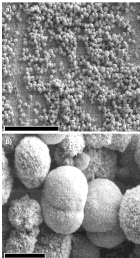
Figure 3. Scanning electron micrographs of precipitates obtained from crystallizations ( 30 \text{ mg L}^{-1} ) at about 4^\circ\text{C} . The spherulike morphology is retained (a), while at higher magnifications (b) differences become visible. The individual crystallites making up the assemblies are no longer rhombohedral, but fluffy and branched. Some bilobed structures are also observed. The scale bars correspond to 200 and 10 \mu\text{m} , respectively.
